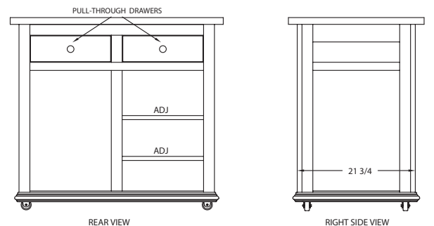
REAR VIEW
